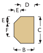
PES3 Jamb Block section
