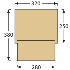
Section through Double Porch Jamb Block.
