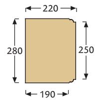
Section through Double Porch Jamb Block.
